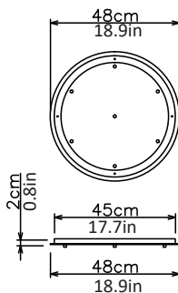
Ceiling Plate
